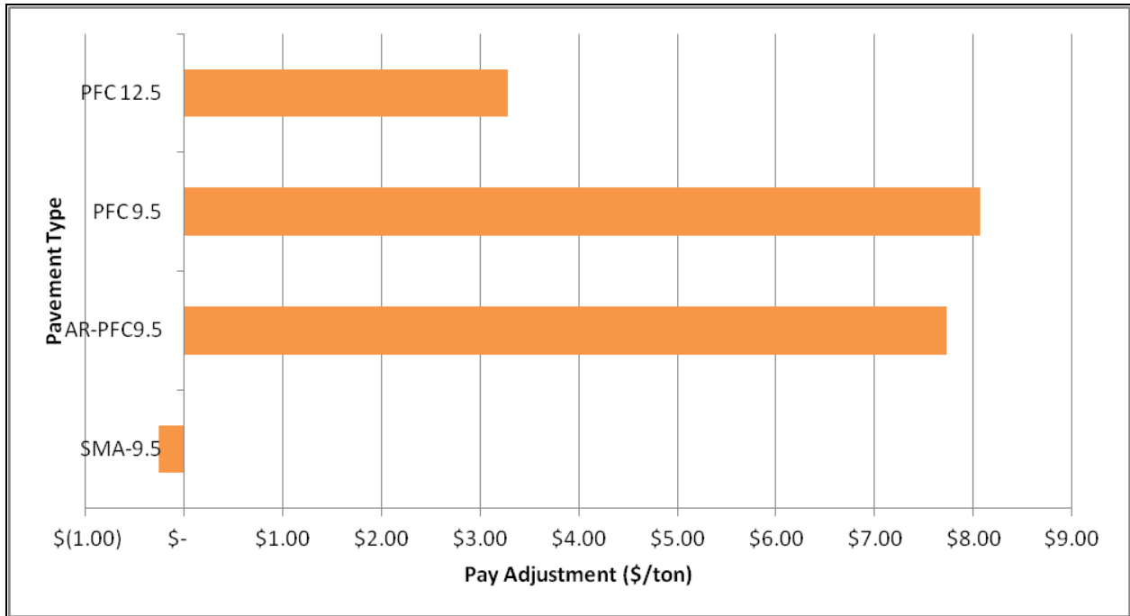
Figure 11. Average pay adjustments for smoothness.
